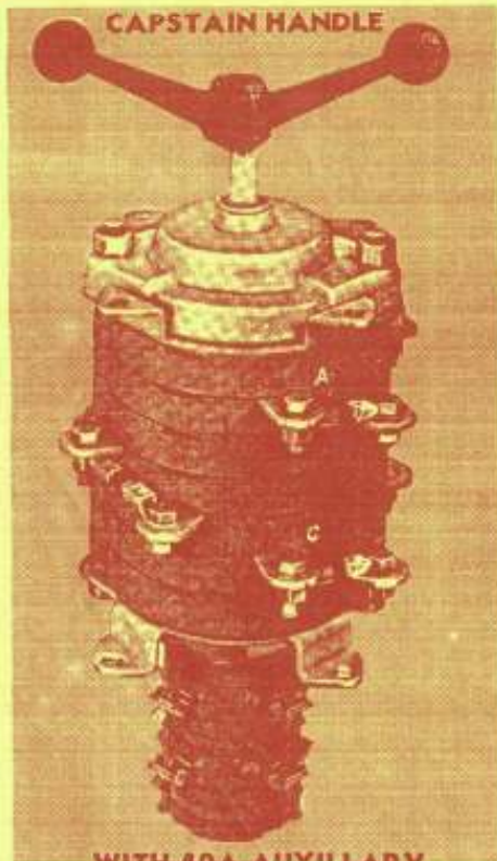
CAPSTAIN HANDLE
