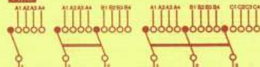
Large Frame Spring Return Type Rotary Switch For Breaker Control application fitted with EE Pistol Grip Handle
